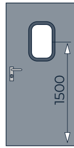
Oblò 300x500 FM L min=700
